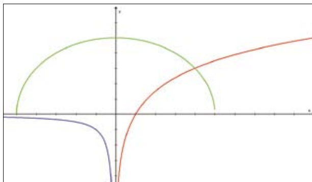
Figur 3: Konkave kurver
